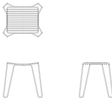
Low Stool TUI-00 W 500 D 440 H 450
